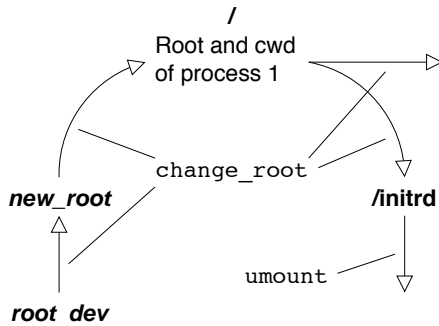
Figure 11: Changing the root file system with change_root .
